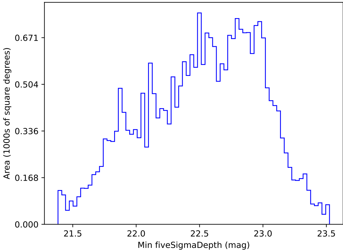
roll_pause_mjdp365_v3.4_10yrs All sky r band: Min fiveSigmaDepth
