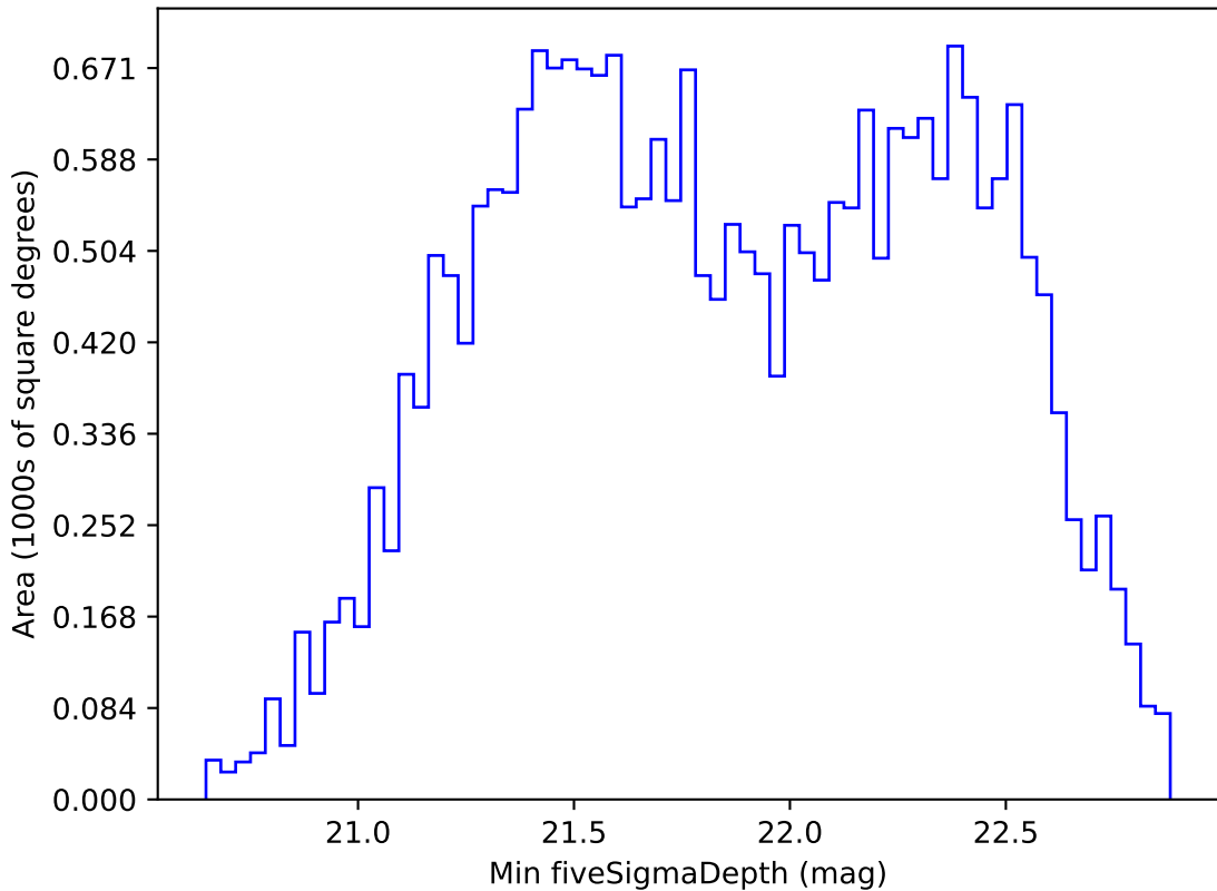
roll_pause_mjdp365_v3.4_10yrs All sky i band: Min fiveSigmaDepth
