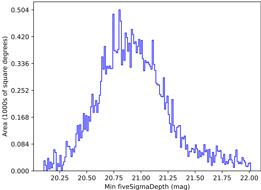
roll_pause_mjdp365_v3.4_10yrs All sky all bands: Min fiveSigmaDepth
