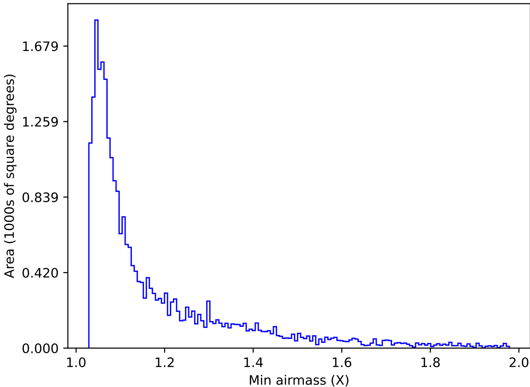
roll_pause_mjdp365_v3.4_10yrs Yr 1 g band: Min airmass
