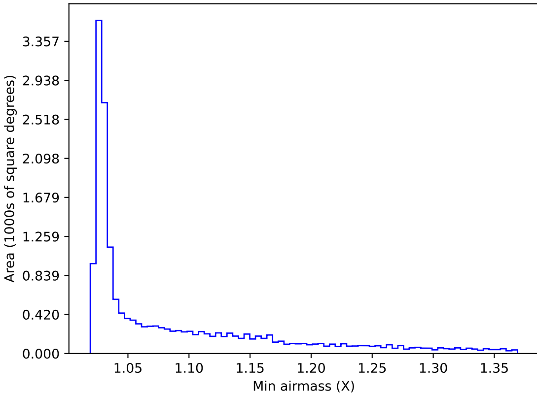
roll_pause_mjdp365_v3.4_10yrs WFD z band: Min airmass
