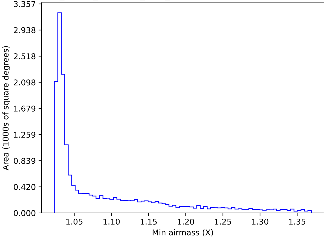
roll_pause_mjdp365_v3.4_10yrs WFD y band: Min airmass
