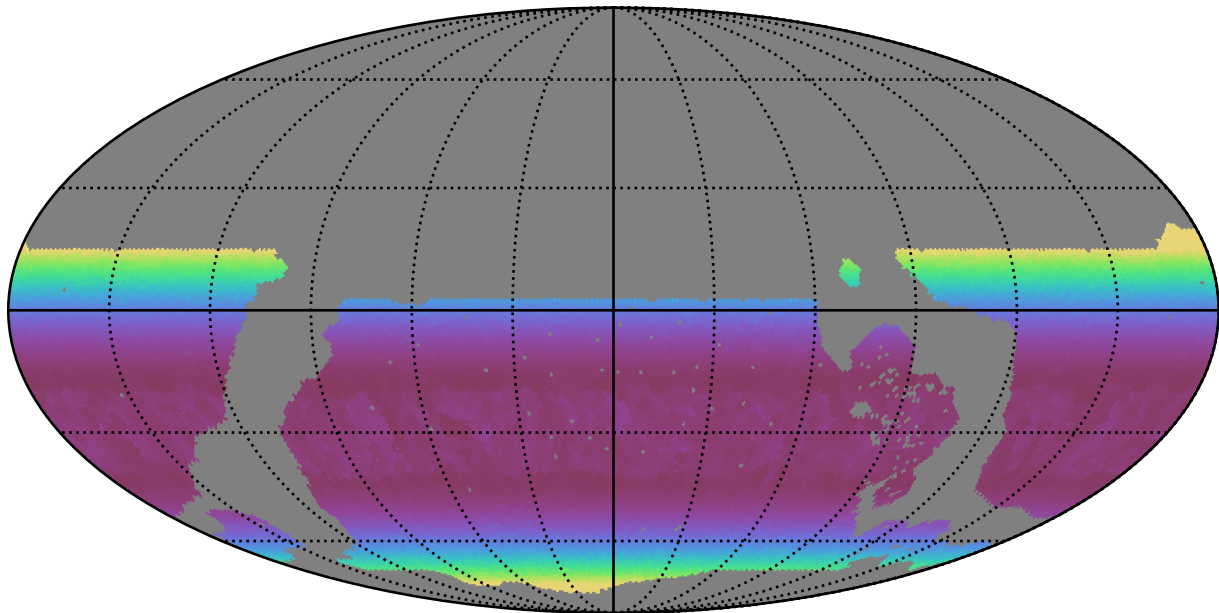
roll_pause_mjdp365_v3.4_10yrs WFD g band: Min airmass
