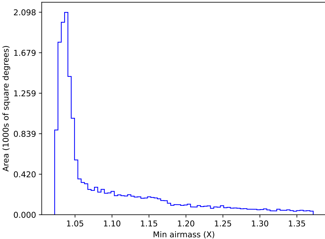
roll_pause_mjdp365_v3.4_10yrs WFD g band: Min airmass
