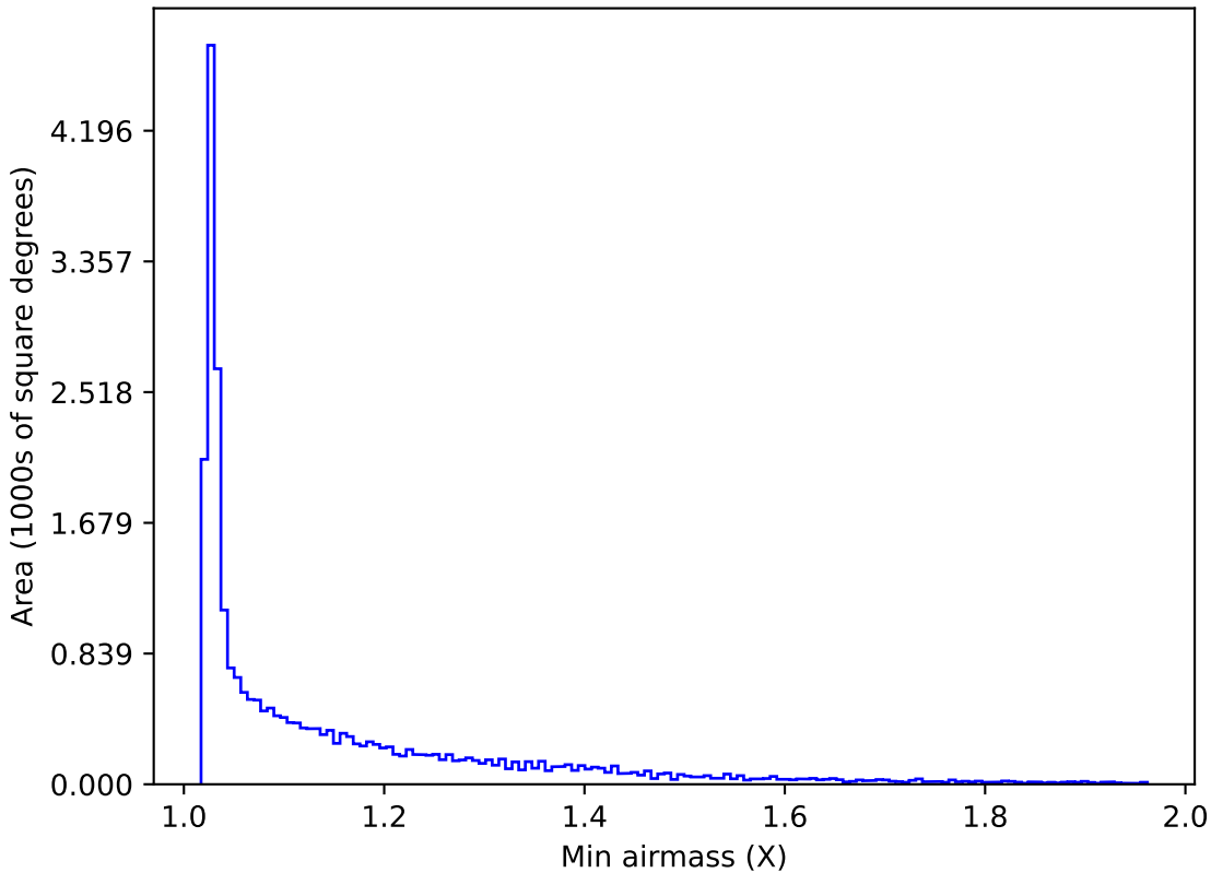
roll_pause_mjdp365_v3.4_10yrs All sky r band: Min airmass
