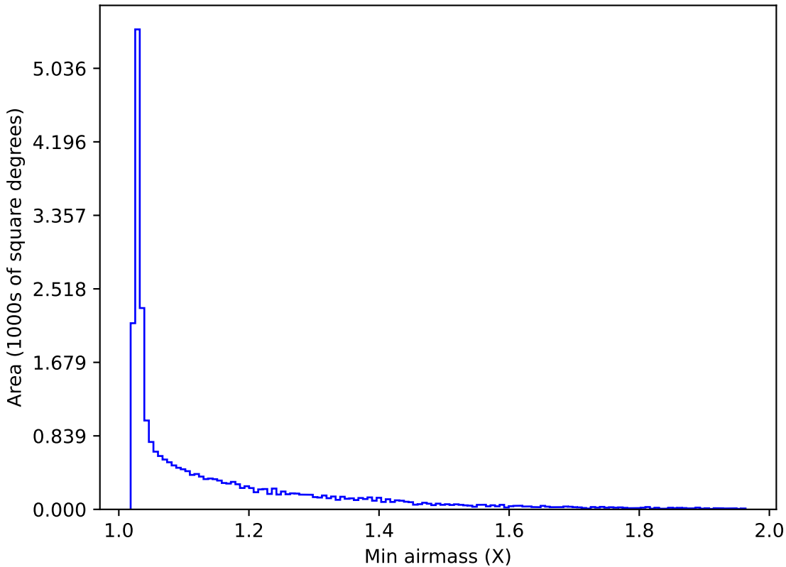
roll_pause_mjdp365_v3.4_10yrs All sky i band: Min airmass
