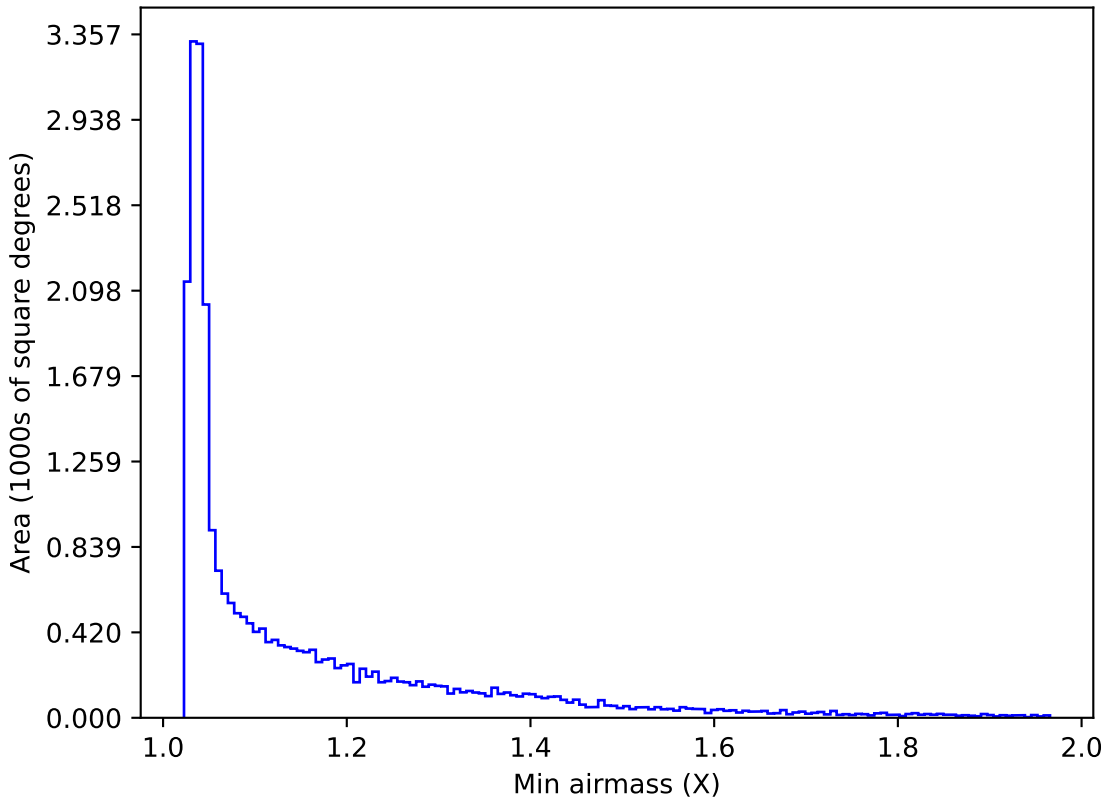
roll_pause_mjdp365_v3.4_10yrs All sky g band: Min airmass
