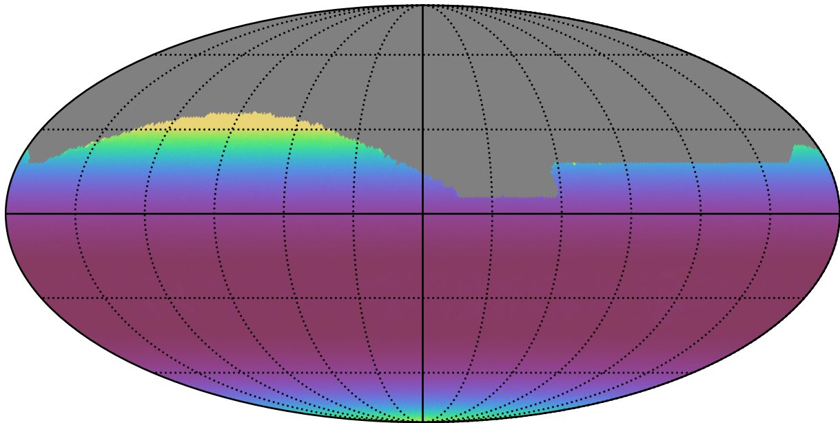
roll_pause_mjdp365_v3.4_10yrs All sky all bands: Min airmass
