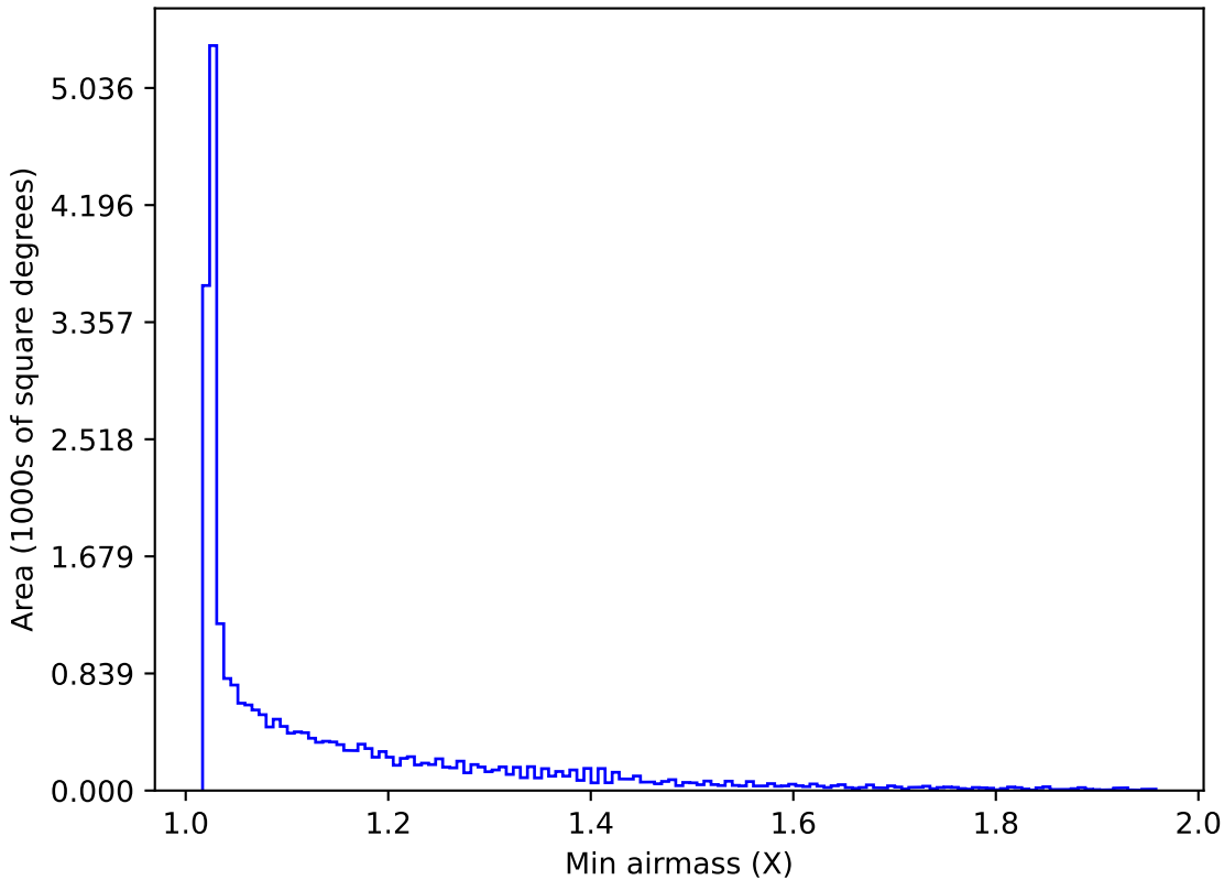
roll_pause_mjdp365_v3.4_10yrs All sky all bands: Min airmass
