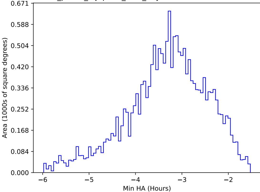
roll_pause_mjdp365_v3.4_10yrs WFD u band: Min HA
