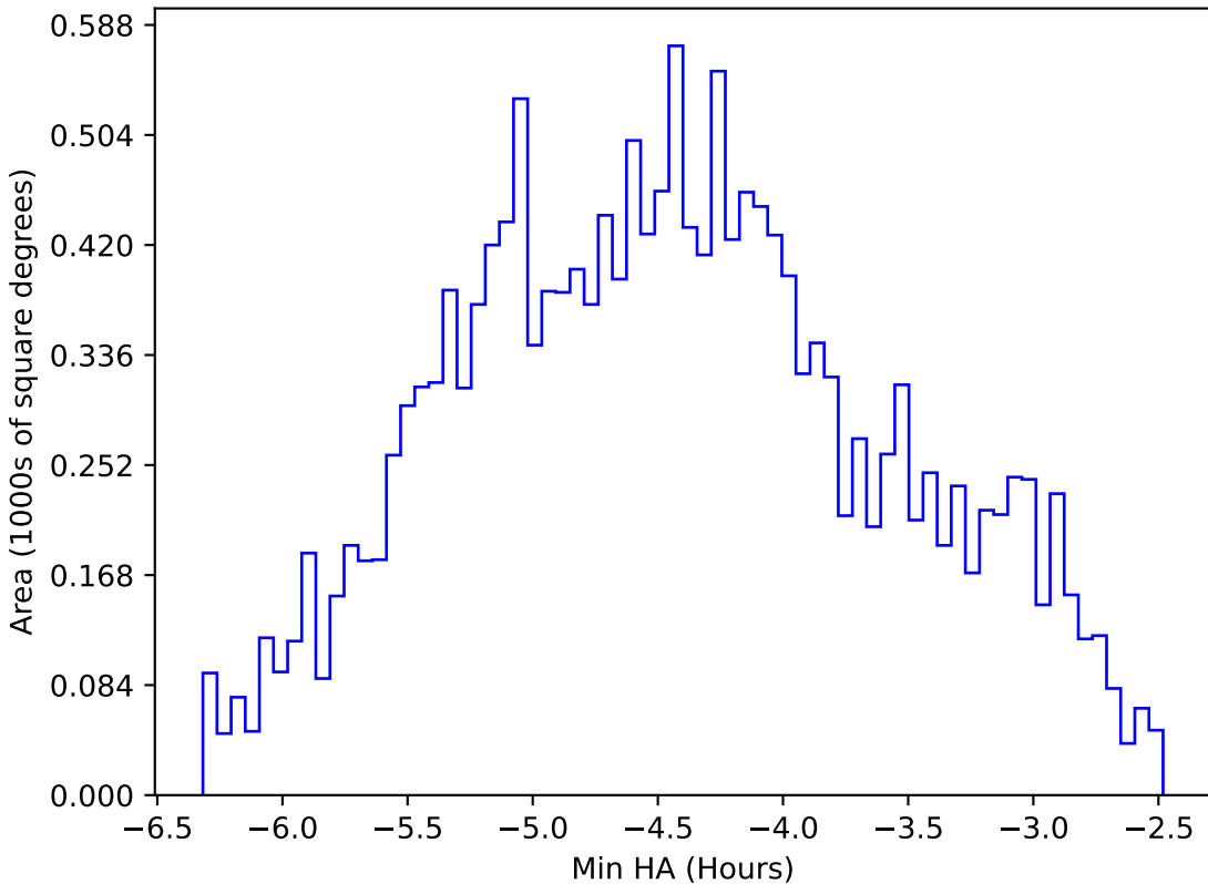
roll_pause_mjdp365_v3.4_10yrs WFD r band: Min HA
