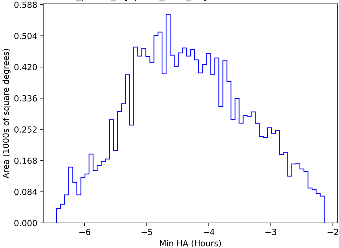
roll_pause_mjdp365_v3.4_10yrs WFD i band: Min HA
