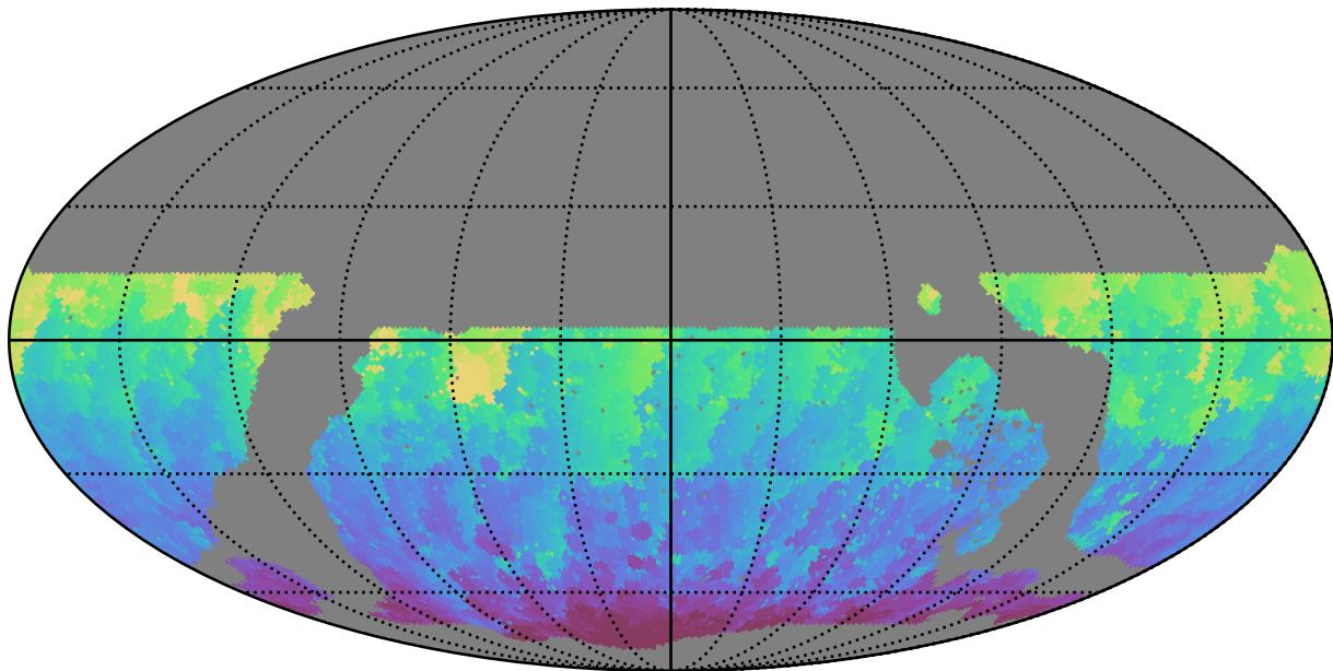
roll_pause_mjdp365_v3.4_10yrs WFD g band: Min HA
