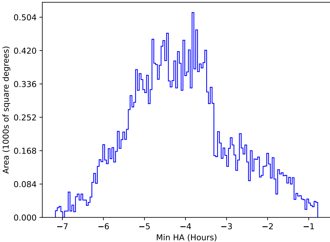
roll_pause_mjdp365_v3.4_10yrs All sky z band: Min HA
