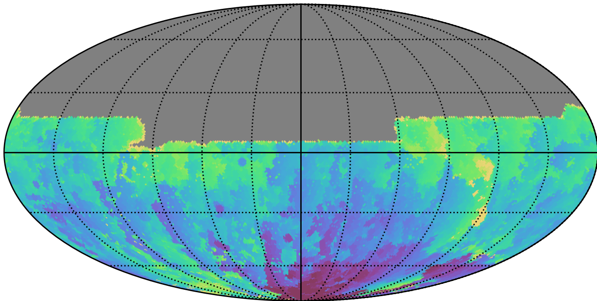
roll_pause_mjdp365_v3.4_10yrs All sky u band: Min HA
