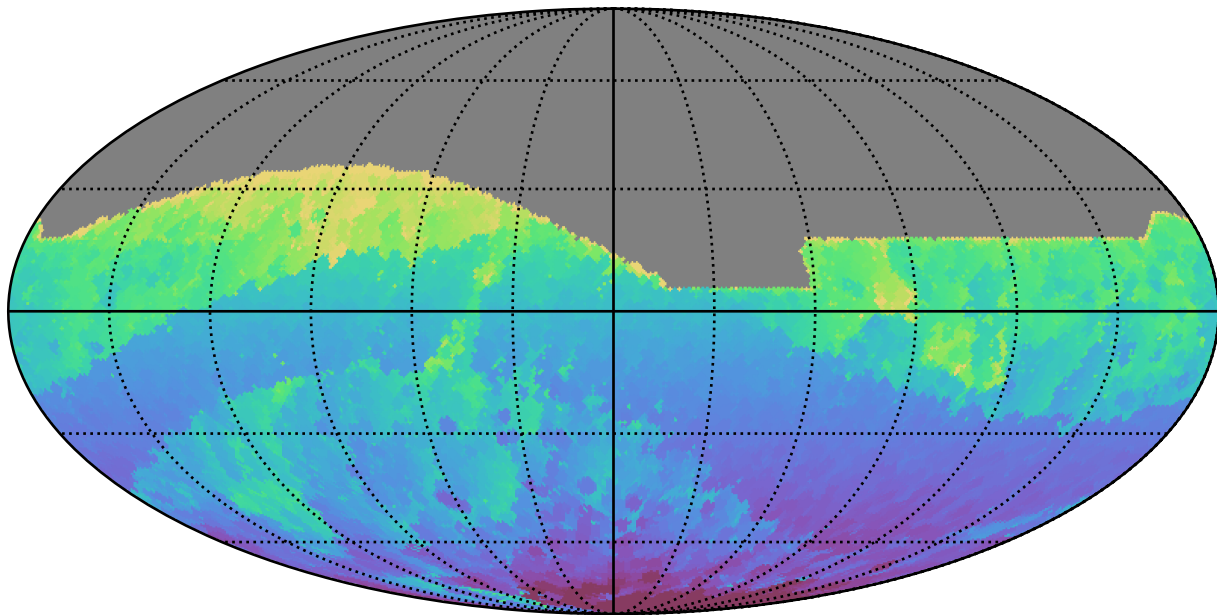
roll_pause_mjdp365_v3.4_10yrs All sky r band: Min HA
