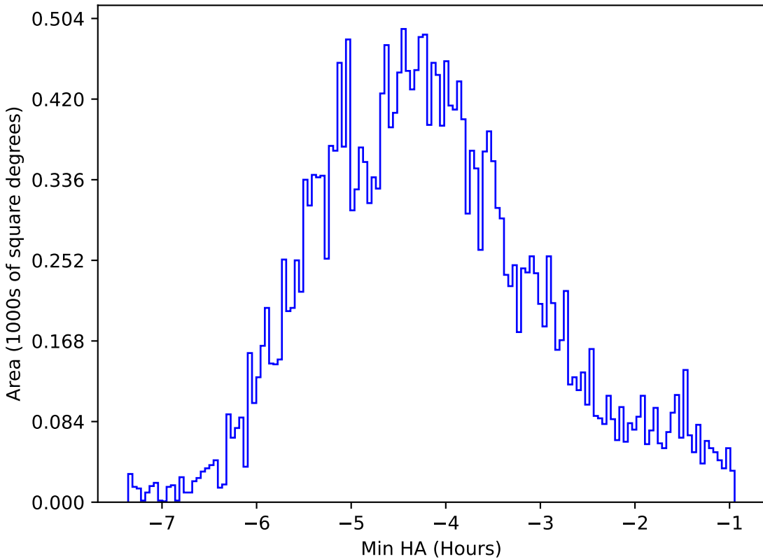
roll_pause_mjdp365_v3.4_10yrs All sky r band: Min HA
