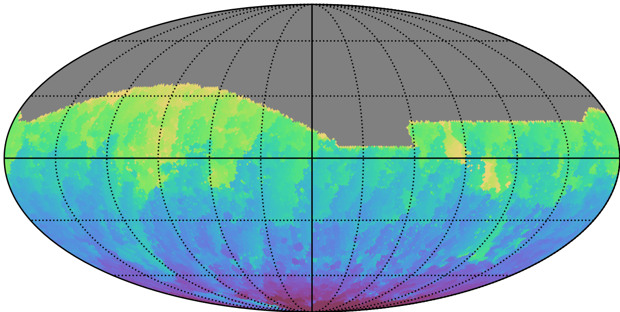
roll_pause_mjdp365_v3.4_10yrs All sky g band: Min HA
