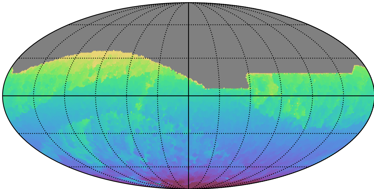
roll_pause_mjdp365_v3.4_10yrs All sky all bands: Min HA
