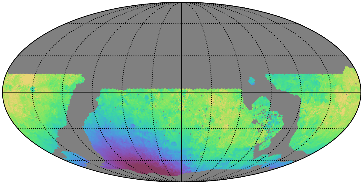
roll_pause_mjdp365_v3.4_10yrs WFD y band: Median solarElong
