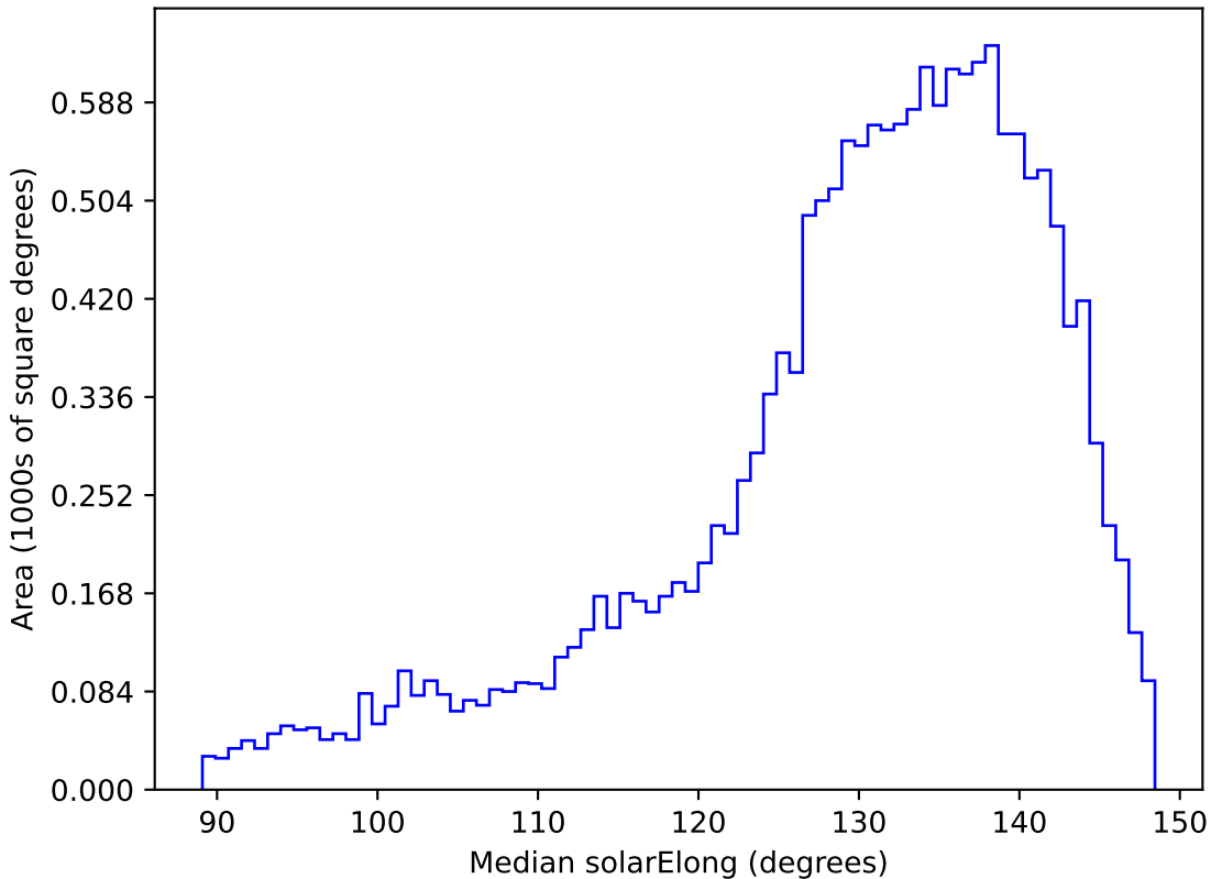
roll_pause_mjdp365_v3.4_10yrs WFD y band: Median solarElong
