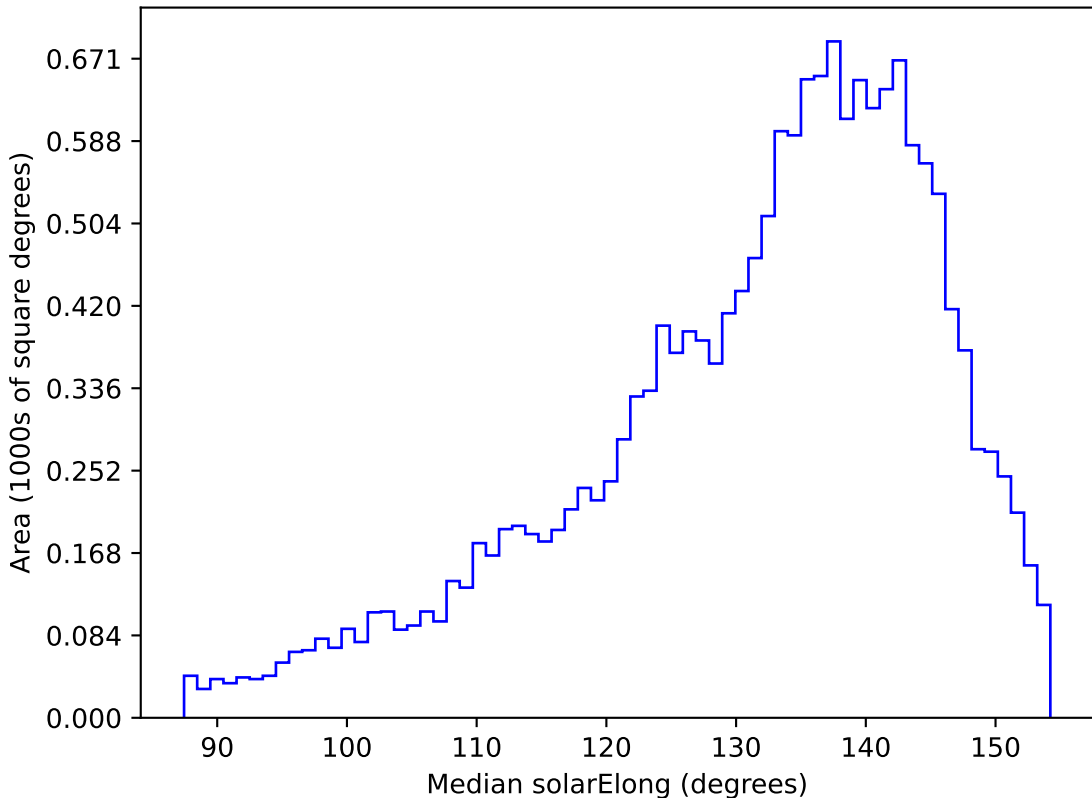
roll_pause_mjdp365_v3.4_10yrs WFD u band: Median solarElong
