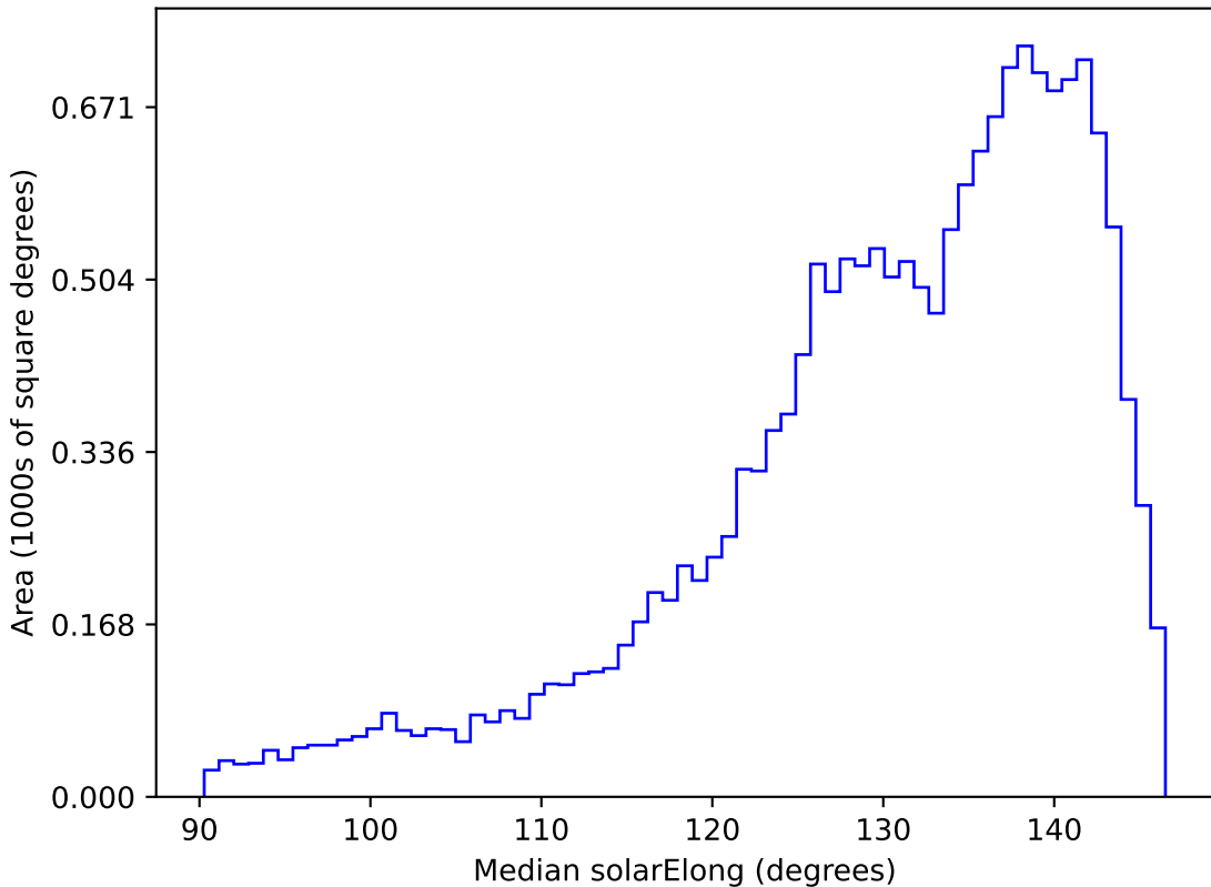
roll_pause_mjdp365_v3.4_10yrs WFD r band: Median solarElong
