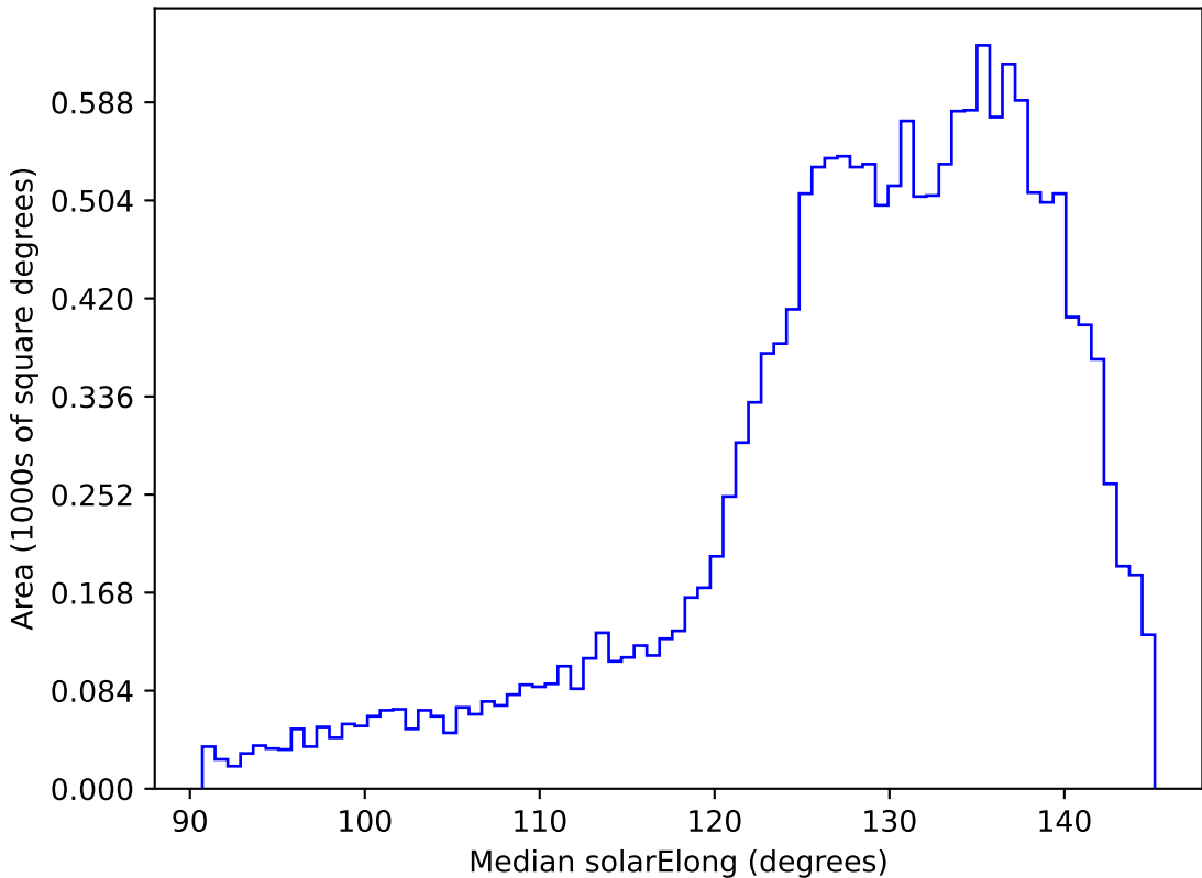
roll_pause_mjdp365_v3.4_10yrs WFD i band: Median solarElong
