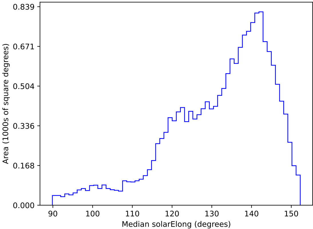
roll_pause_mjdp365_v3.4_10yrs WFD g band: Median solarElong
