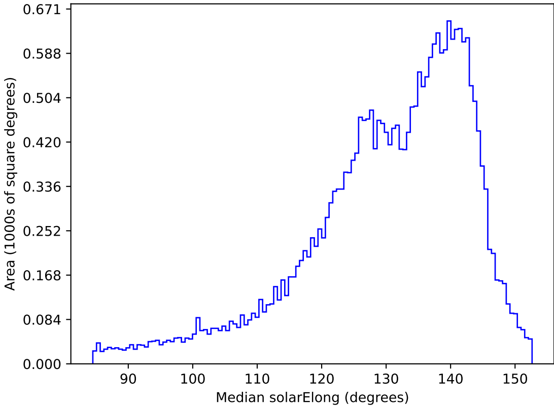
roll_pause_mjdp365_v3.4_10yrs All sky r band: Median solarElong
