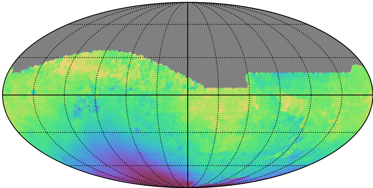
roll_pause_mjdp365_v3.4_10yrs All sky i band: Median solarElong
