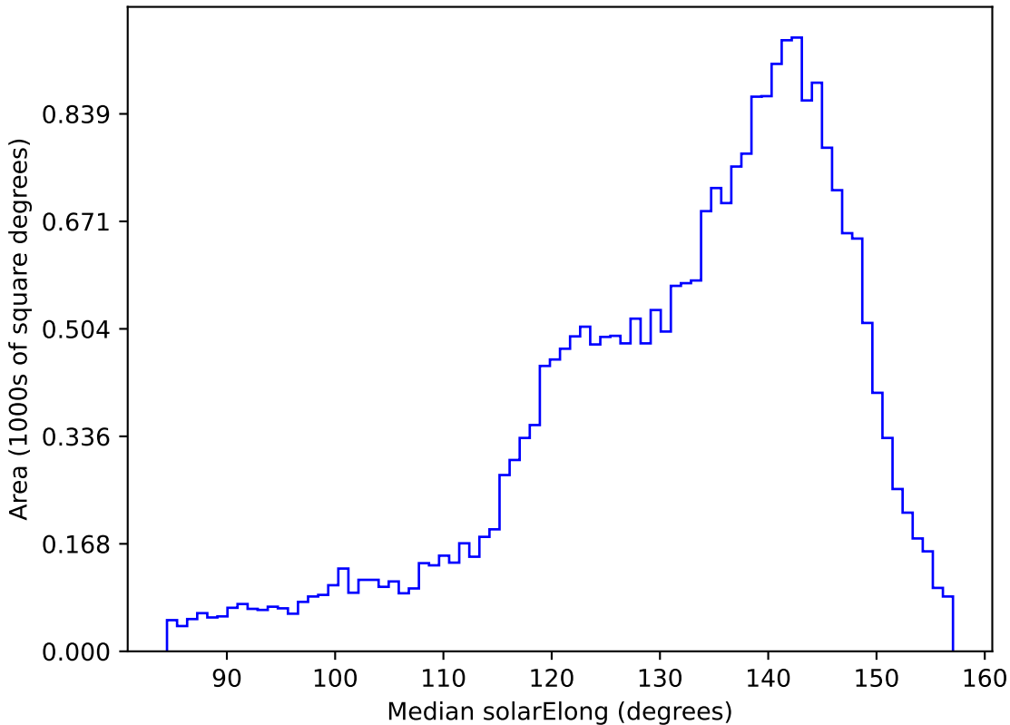
roll_pause_mjdp365_v3.4_10yrs All sky g band: Median solarElong
