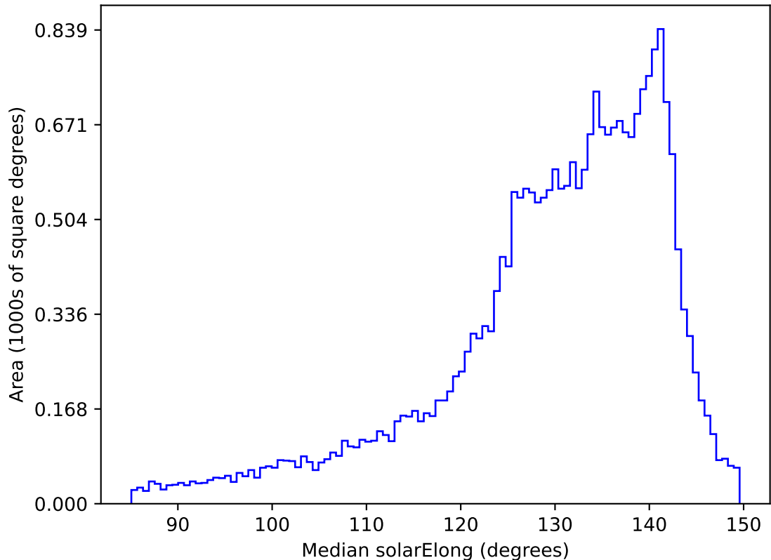
roll_pause_mjdp365_v3.4_10yrs All sky all bands: Median solarElong
