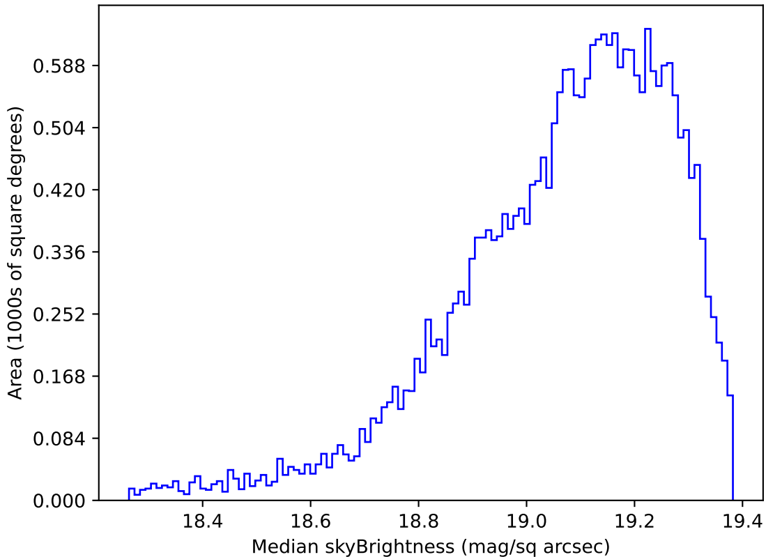
roll_pause_mjdp365_v3.4_10yrs Yr 1 z band: Median skyBrightness
