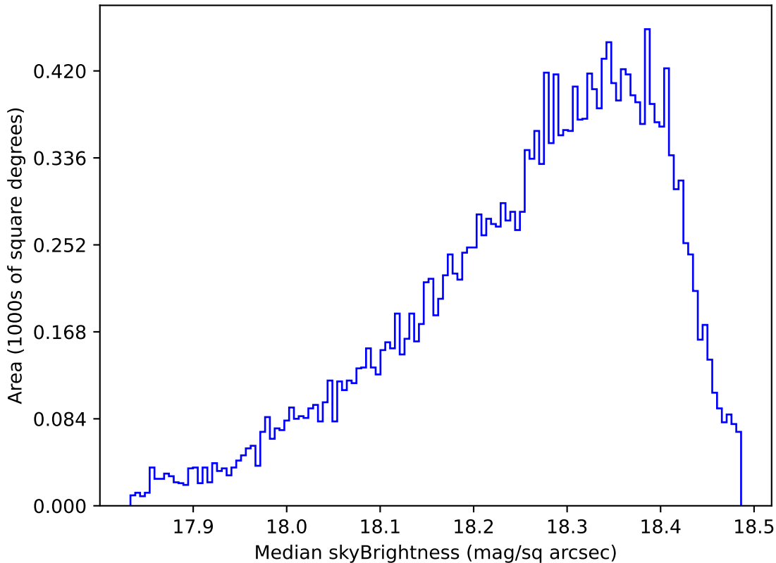
roll_pause_mjdp365_v3.4_10yrs Yr 1 y band: Median skyBrightness
