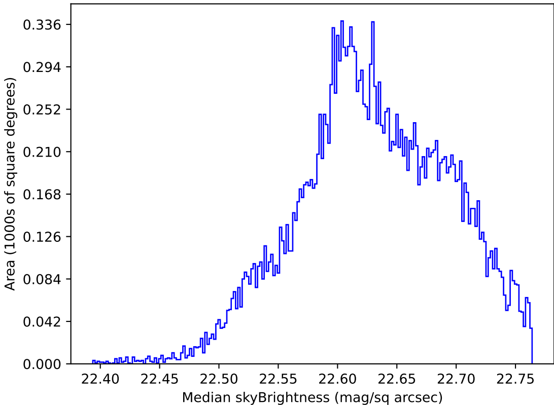
roll_pause_mjdp365_v3.4_10yrs Yr 1 u band: Median skyBrightness
