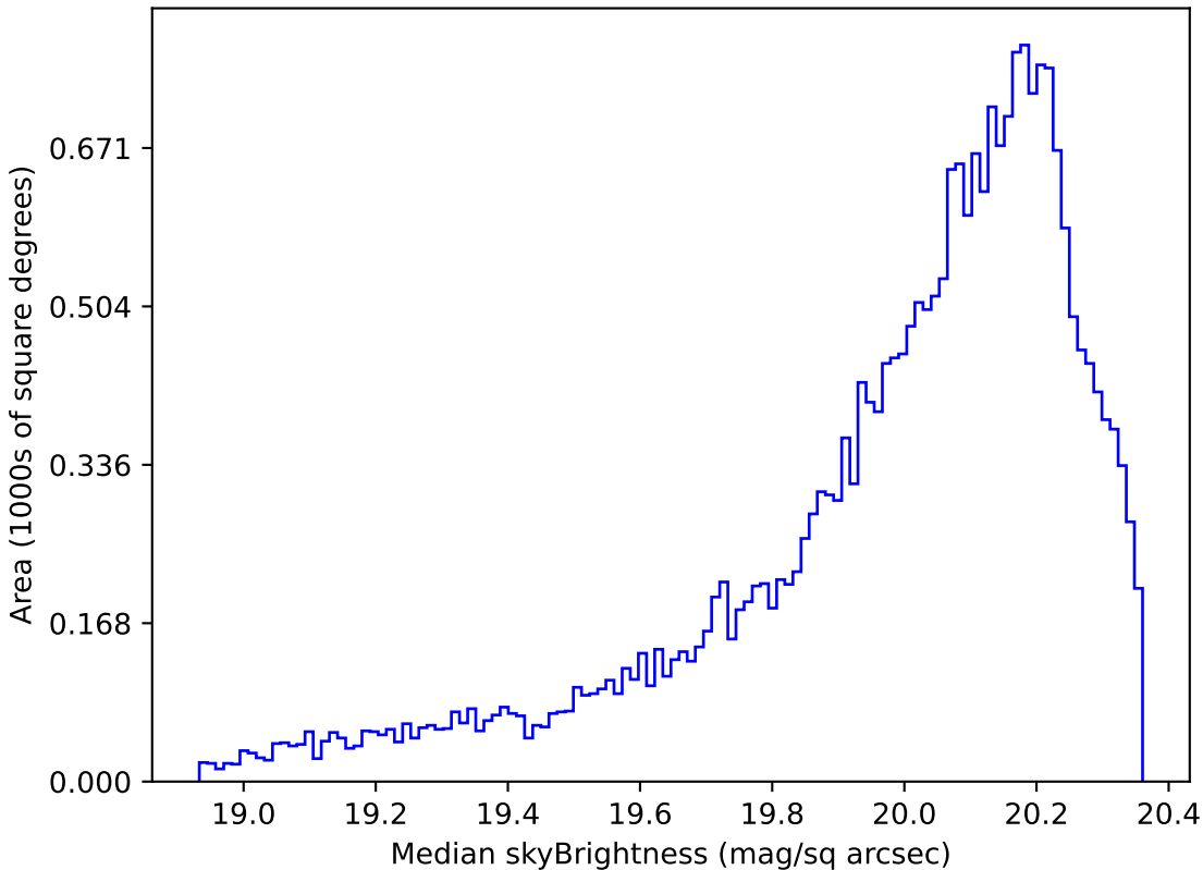
roll_pause_mjdp365_v3.4_10yrs Yr 1 i band: Median skyBrightness
