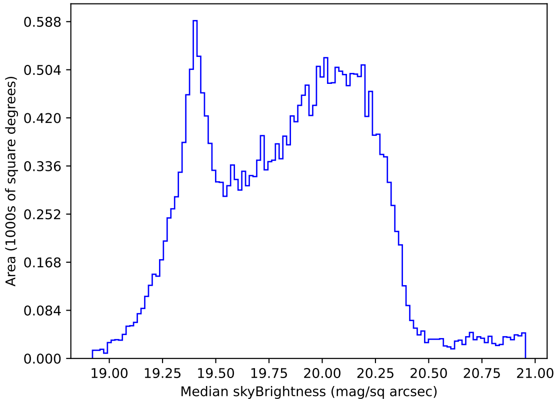
roll_pause_mjdp365_v3.4_10yrs Yr 1 all bands: Median skyBrightness
