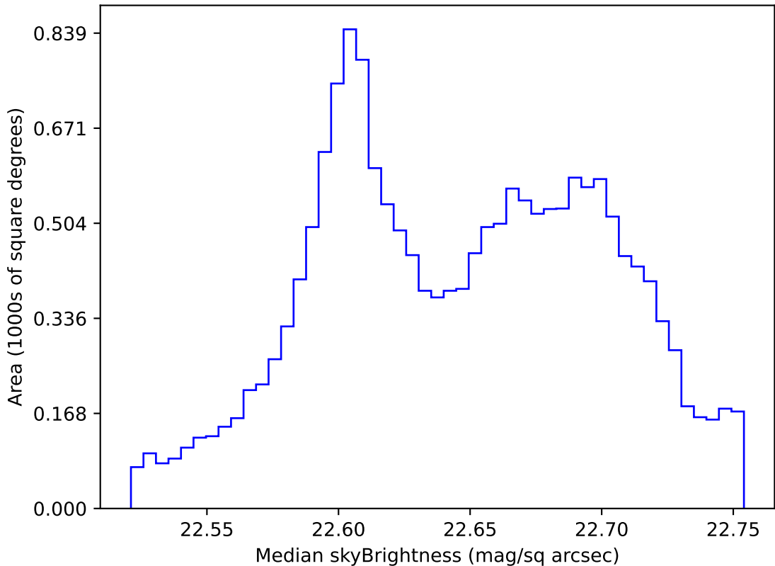
roll_pause_mjdp365_v3.4_10yrs WFD u band: Median skyBrightness
