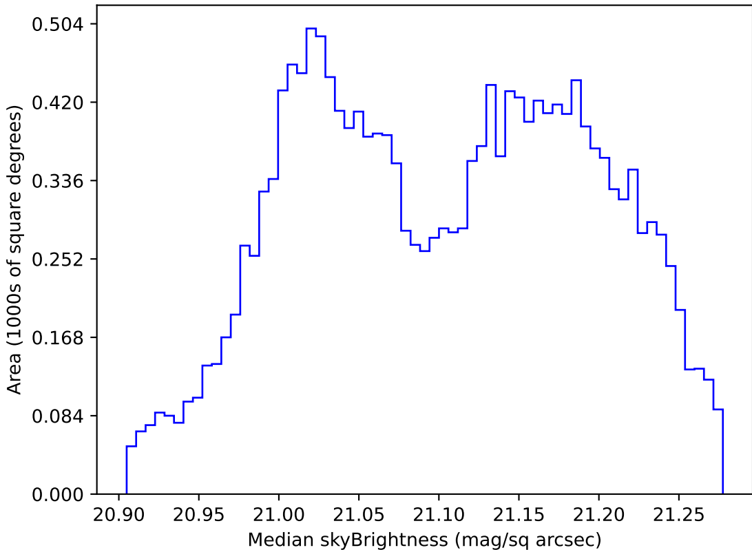
roll_pause_mjdp365_v3.4_10yrs WFD r band: Median skyBrightness
