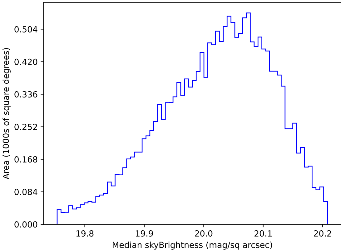
roll_pause_mjdp365_v3.4_10yrs WFD i band: Median skyBrightness
