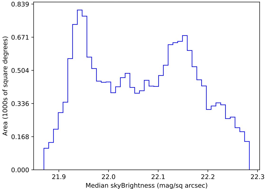
roll_pause_mjdp365_v3.4_10yrs WFD g band: Median skyBrightness
