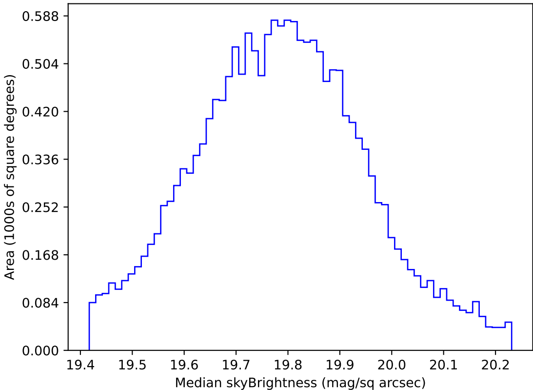
roll_pause_mjdp365_v3.4_10yrs WFD all bands: Median skyBrightness
