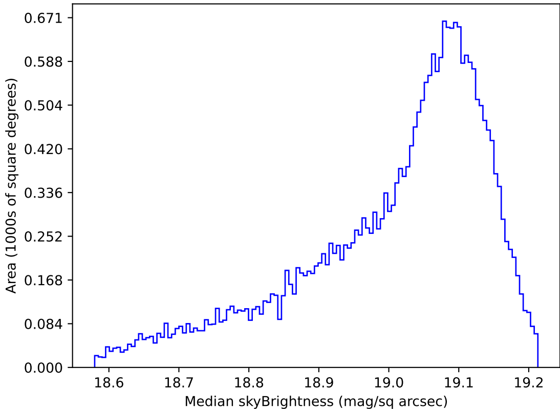
roll_pause_mjdp365_v3.4_10yrs All sky z band: Median skyBrightness
