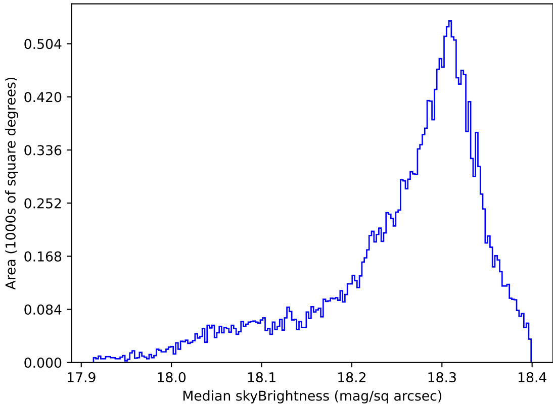
roll_pause_mjdp365_v3.4_10yrs All sky y band: Median skyBrightness
