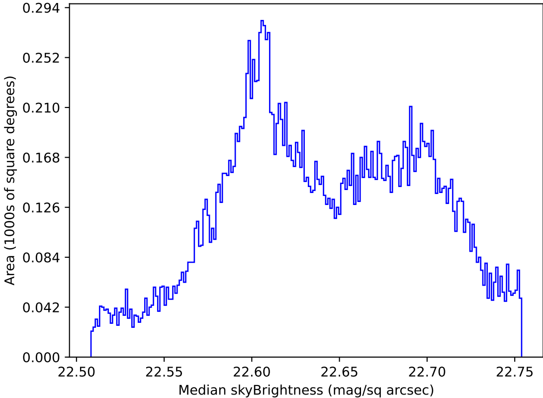
roll_pause_mjdp365_v3.4_10yrs All sky u band: Median skyBrightness
