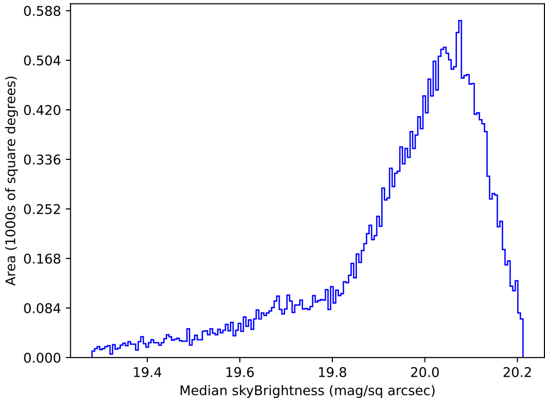
roll_pause_mjdp365_v3.4_10yrs All sky i band: Median skyBrightness
