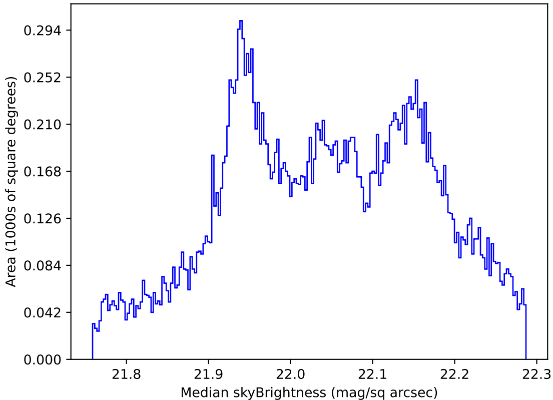
roll_pause_mjdp365_v3.4_10yrs All sky g band: Median skyBrightness
