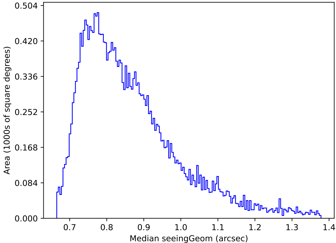
roll_pause_mjdp365_v3.4_10yrs Yr 1 r band: Median seeingGeom
