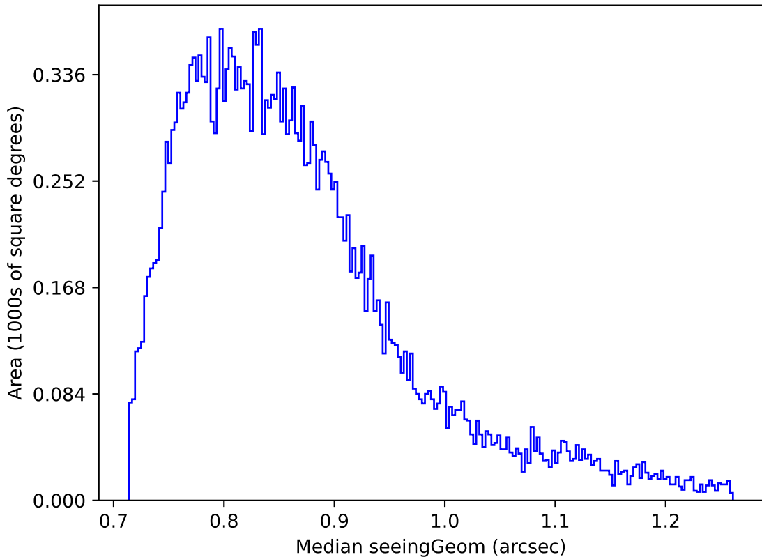
roll_pause_mjdp365_v3.4_10yrs Yr 1 all bands: Median seeingGeom
